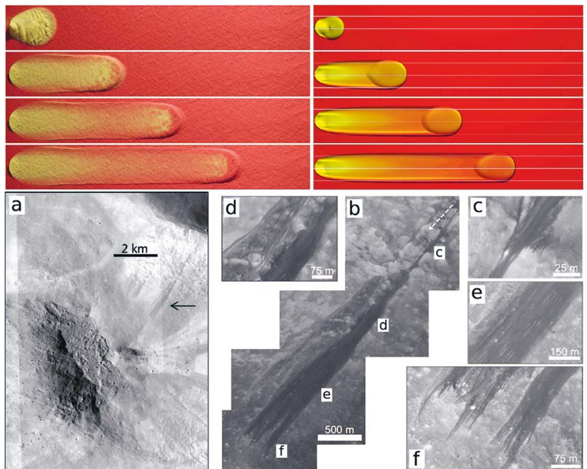
► FIG. 3: Steady travelling wave propagating on an erodible layer of constant thickness. Experiments (top left panel), corresponding numerical simulation via a depth-averaged model with viscous terms and a non-monotonic friction law (top right panel). Debris-flow deposit in the Virtanen F crater interpreted to result from the propagation of erosion-deposition waves (bottom panel) (from Viroulet et al. 2019).
